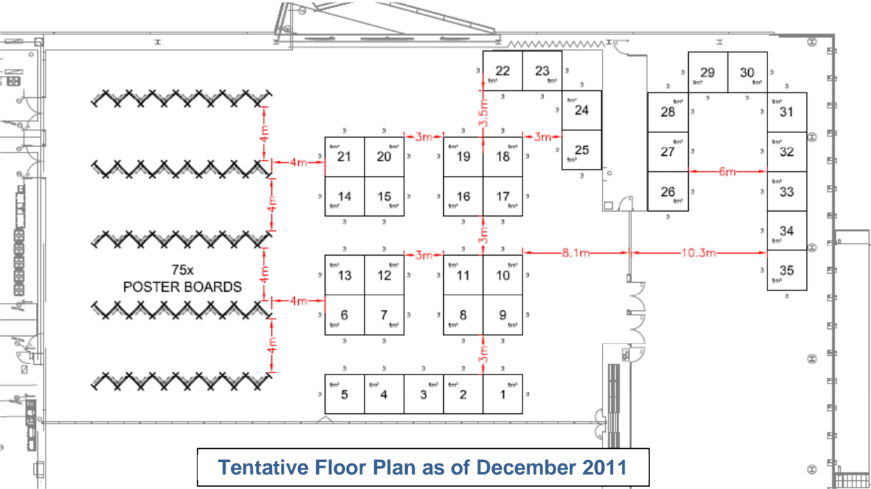
Level 2 of Melbourne Convention Centre Session Rooms Exhibition Area
